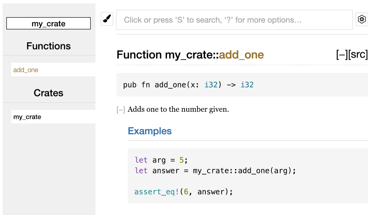
Figure 14-1: HTML documentation for the add_one function
