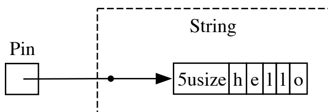
Figure 17-8: Pinning a String ; the dotted line indicates that the String implements the Unpin trait, and thus is not pinned.
