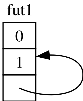
Figure 17-4: A self-referential data type.
